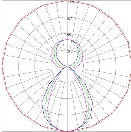
Maximum Candela = 1099 Located At Horizontal Angle = 0, Vertical Angle = 0 # 1 - Vertical Plane Through Horizontal Angles (0 - 180) (Through Max. Cd) : BLUE # 2 - Vertical Plane Through Horizontal Angles (45 - 225) : GREEN # 3 - Vertical Plane Through Horizontal Angles (90 - 270) : MAGENTA # 4 - Horizontal Cone Through Vertical Angle (0) (Through Max. Cd) : RED
