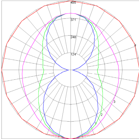
Maximum Candela = 495 Located At Horizontal Angle = 0, Vertical Angle = 0 # 1 - Vertical Plane Through Horizontal Angles (0 - 180) (Through Max. Cd) : BLUE # 2 - Vertical Plane Through Horizontal Angles (45 - 225) : GREEN # 3 - Vertical Plane Through Horizontal Angles (90 - 270) : MAGENTA # 4 - Horizontal Cone Through Vertical Angle (0) (Through Max. Cd) : RED
