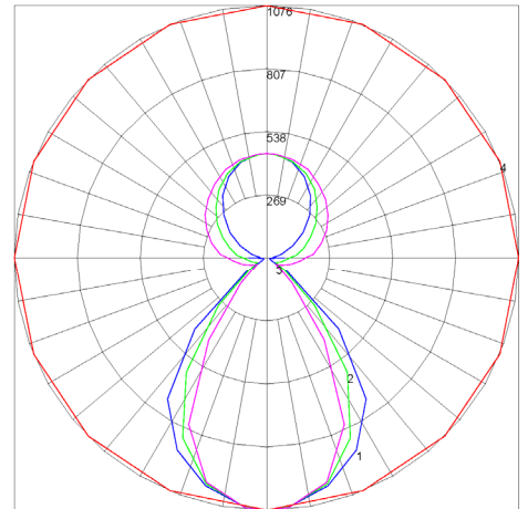
Maximum Candela = 1076 Located At Horizontal Angle = 0, Vertical Angle = 0 # 1 - Vertical Plane Through Horizontal Angles (0 - 180) (Through Max. Cd) : BLUE # 2 - Vertical Plane Through Horizontal Angles (45 - 225) : GREEN # 3 - Vertical Plane Through Horizontal Angles (90 - 270) : MAGENTA # 4 - Horizontal Cone Through Vertical Angle (0) (Through Max. Cd) : RED
